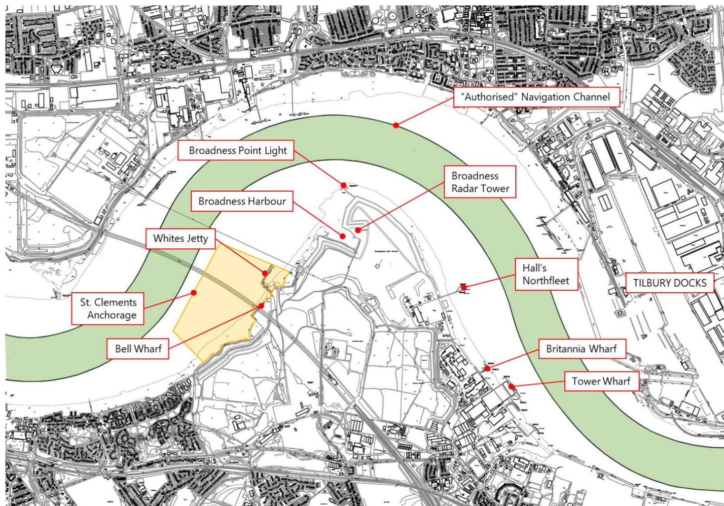
Figure 17.16: Location of marine infrastructure on the Swanscombe Peninsula.
